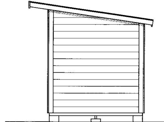
GAVELFASAD 1
