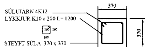
SNID H-H 1:20
