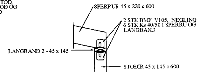
SNID C-C 1:20
