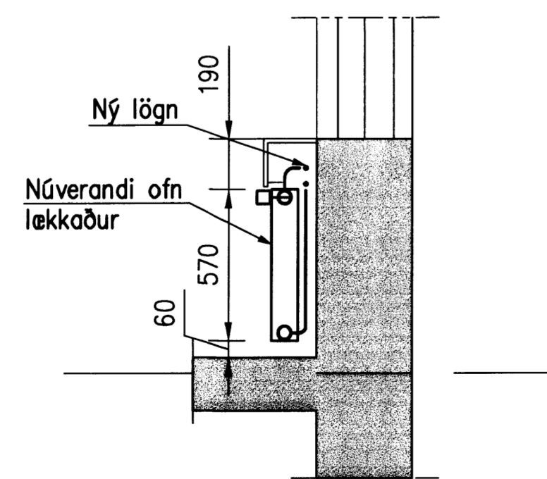
SNID A 1:20
