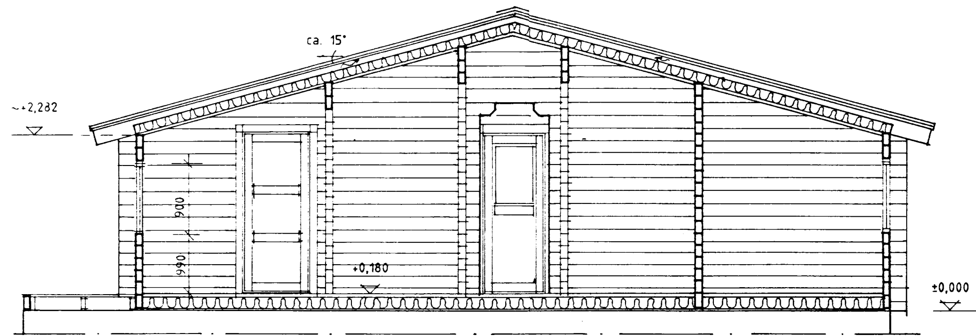
CROSS SECTION A-A 1:50
