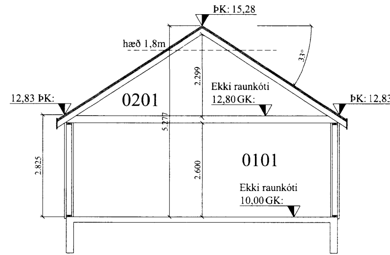
SNID C-C
