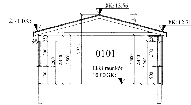
SNID B-B
