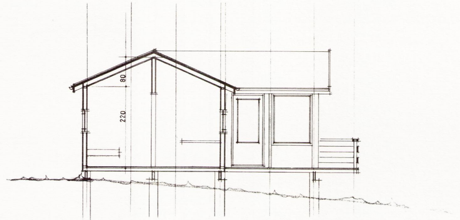
SNID M 1:50
