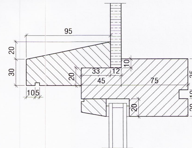
ÞVERSNID KARMS/VATNSBRETTIS 1:2
