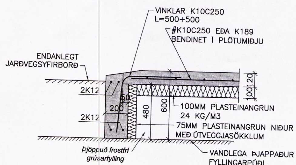
B SNEIÐING 01 Mkv. 1/20
