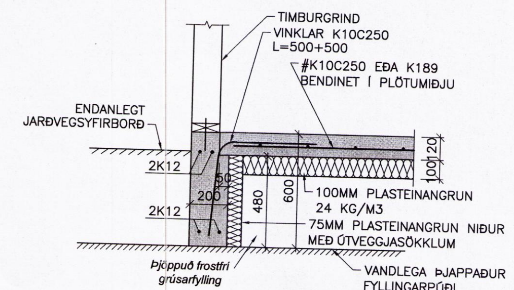
A SNEIÐING 01 Mkv. 1/20
