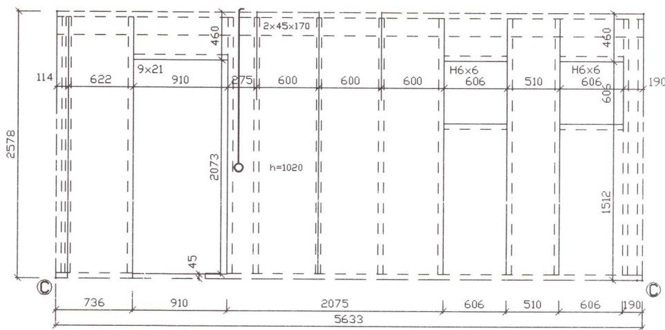
VEGGEINING E4 1:50
