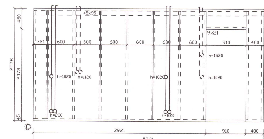
VEGGEINING E6 1:50
