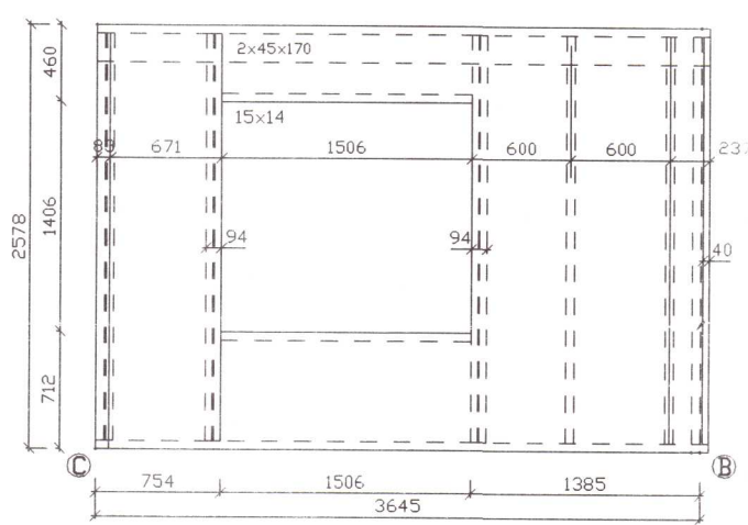
VEGGEINING E5 1:50
