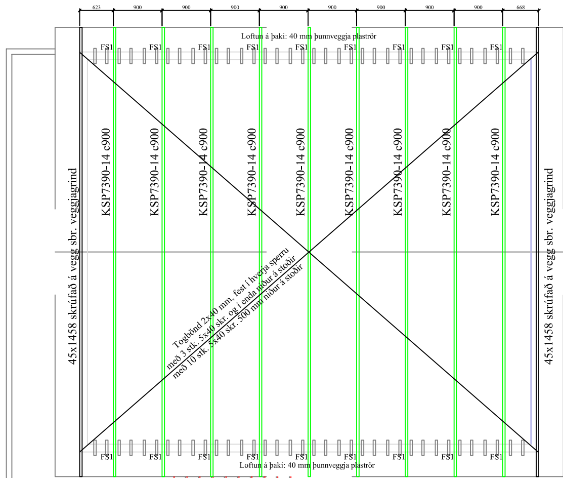
Þakplan - sperrur
