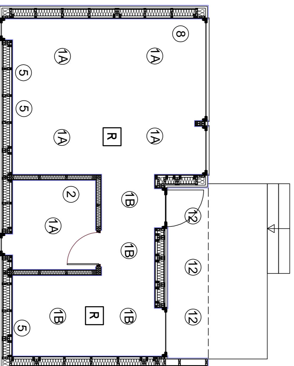
GRUNNMÝND LAMPAPLAN MKV 1:50
