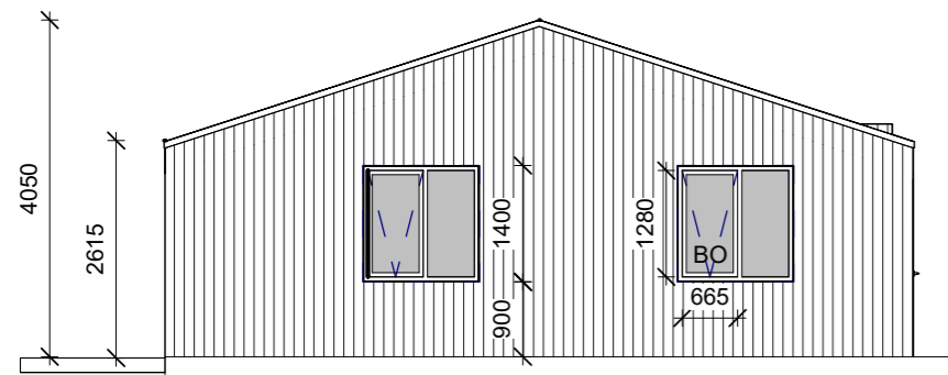
Austur 1: 100
