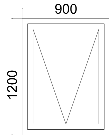
Gluggi G1 3 stk m björgunaropi
