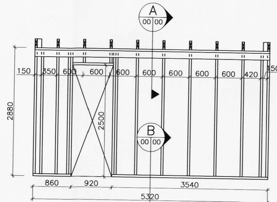
VEGGUR 2 1:50
