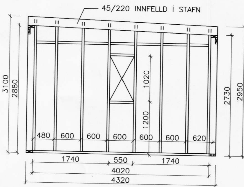
VEGGUR 3 1:50
