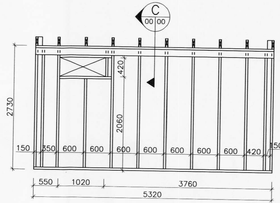
VEGGUR 1 1:50
