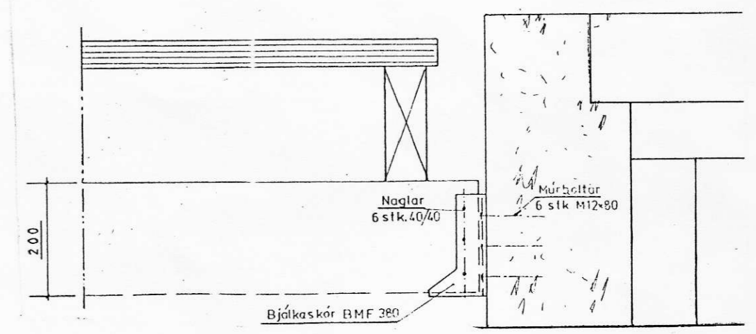
Snid X-X 1:7
