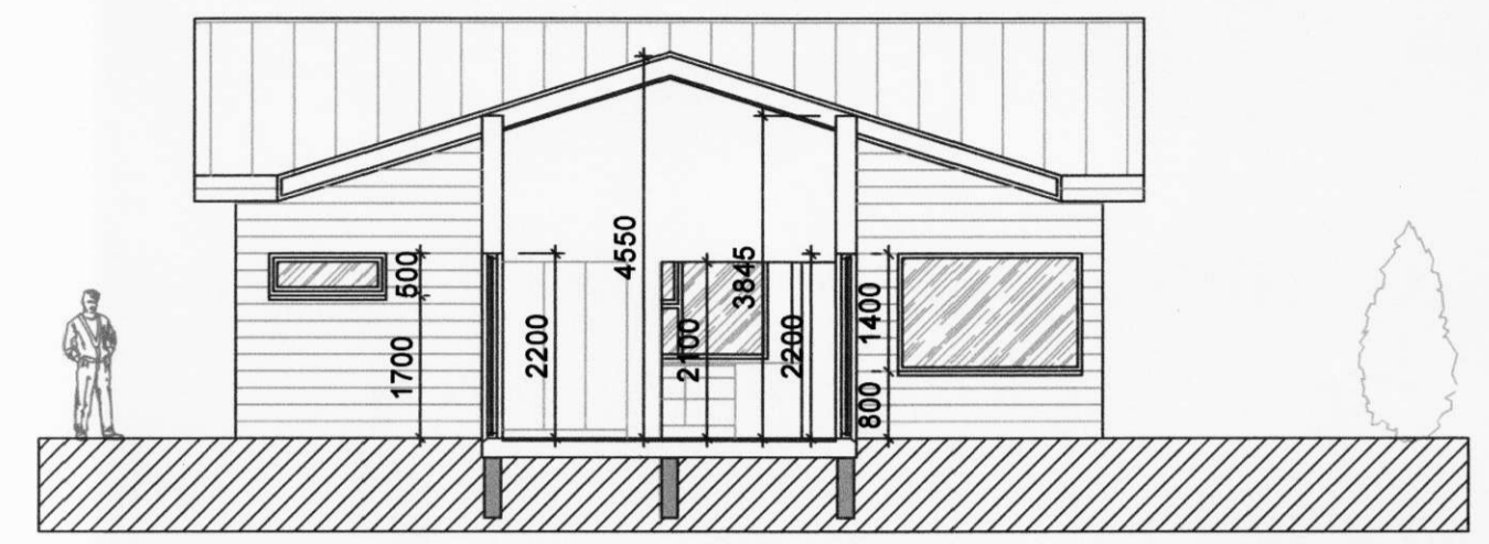
SNEIÐING X-X 1:100
