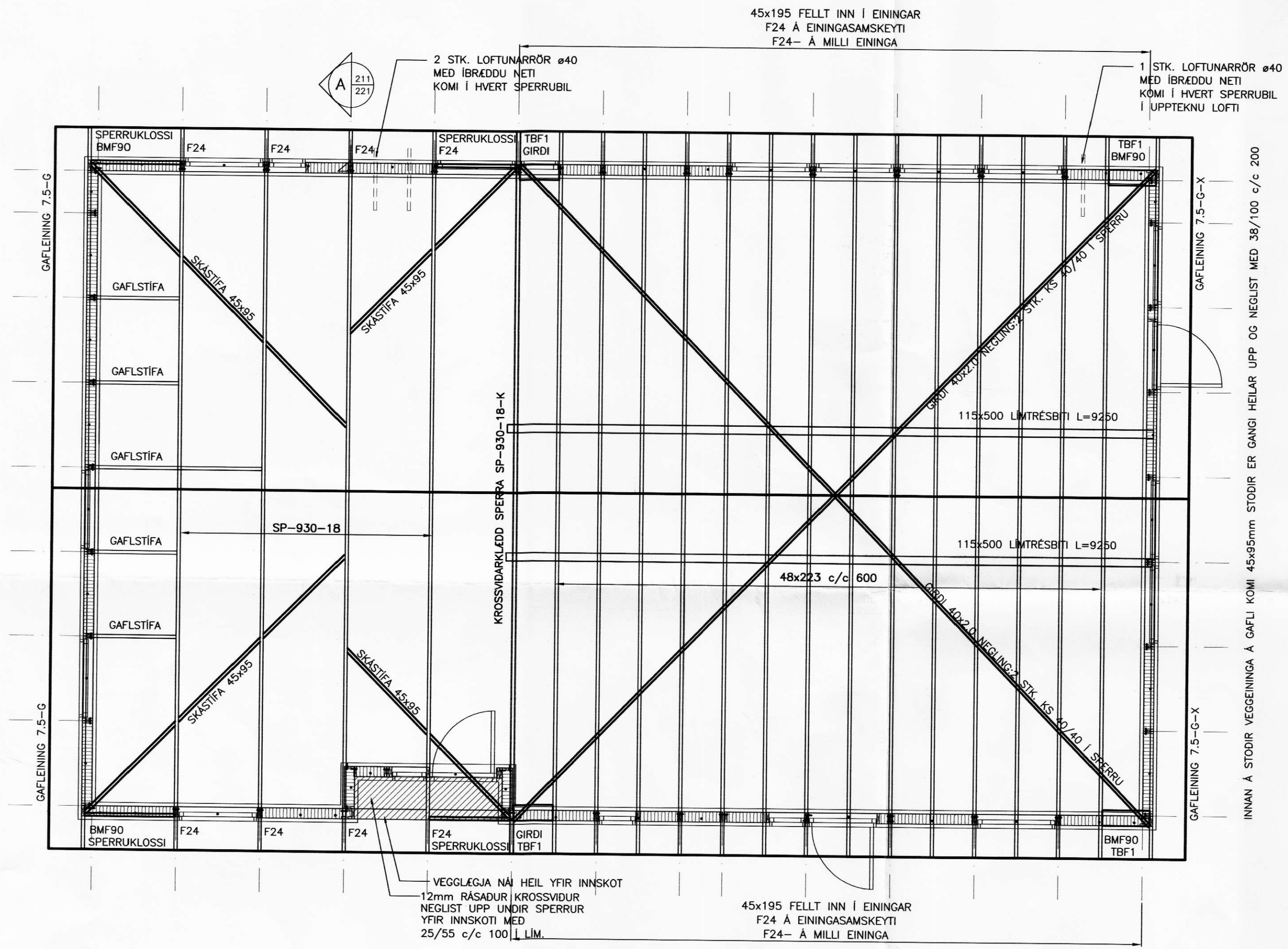
ÞAKPLAN MKV. 1:50
